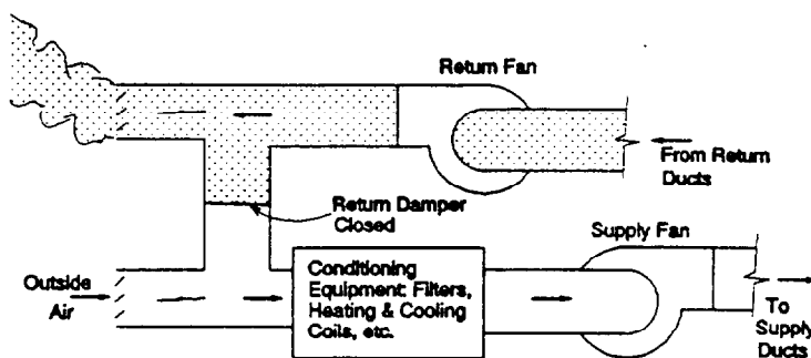
Figure 5. HVAC System With Recirculation Capability in the Smoke Control Mode.
